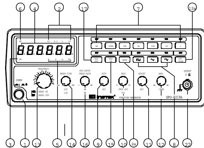
● Fig 4.1 FRONT PANEL
